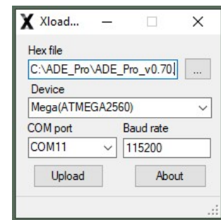
Figure 2: Xloader Program
